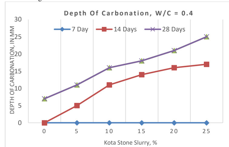
Fig. 7 Depth of Carbonation (Water Cement Ratio = 0.40)
