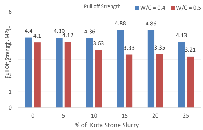
Fig. 5 Pull-Off Strength (Water Cement Ratio =0.40 and 0.50)
