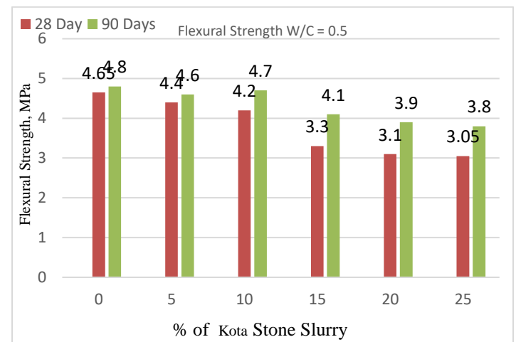
Fig. 4 Flexural Strength (Water Cement Ratio = 0.50)
