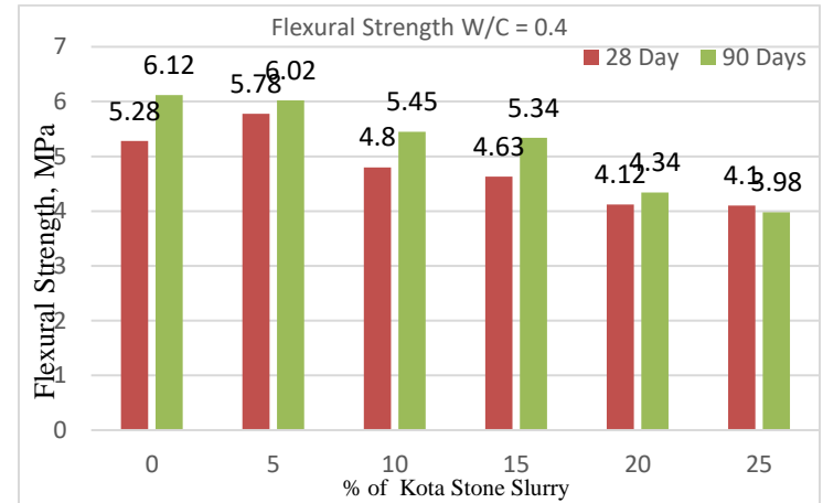
Fig.3 Flexural Strength (Water Cement Ratio = 0.40)
