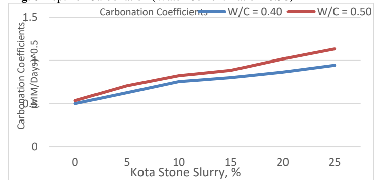
Fig. 9 Carbonation Coefficients (Water Cement Ratio = 0.40 and 0.50)
