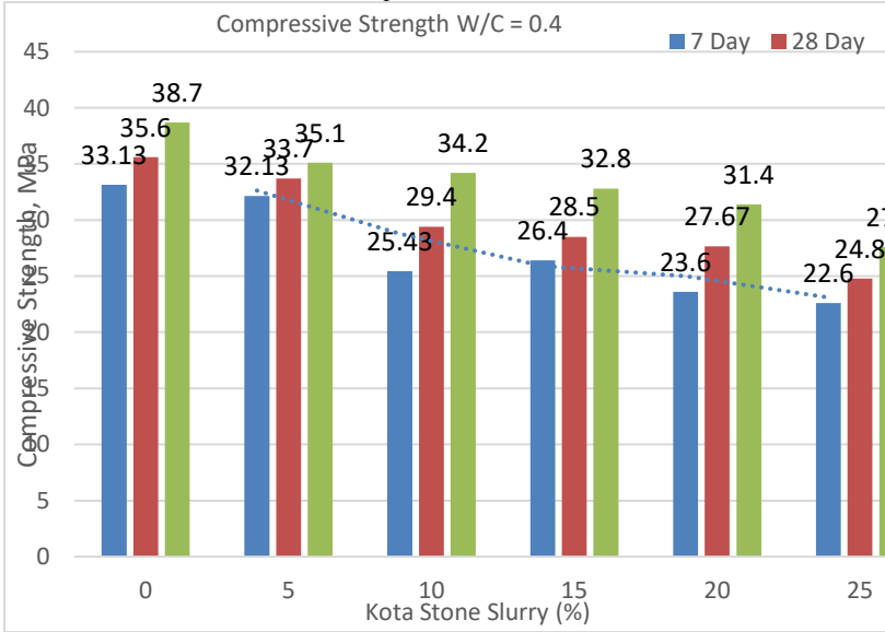
Fig. 1 Compressive Strength (Water Cement Ratio = 0.40)
