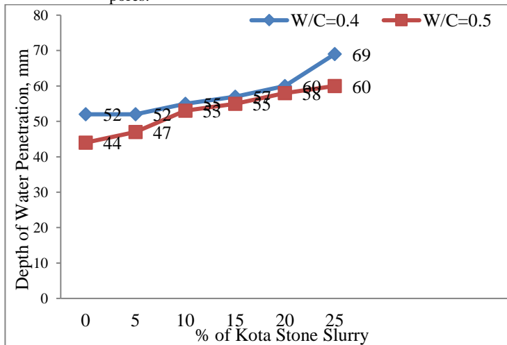
Fig. 6 Depth of Water Penetration, DIN 1048 Permeability Test (Water Cement Ratio = 0.40 and 0.50)
