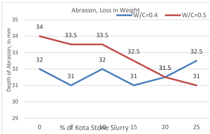
Fig. 10 Depth of Abrasion, Abrasion Test
